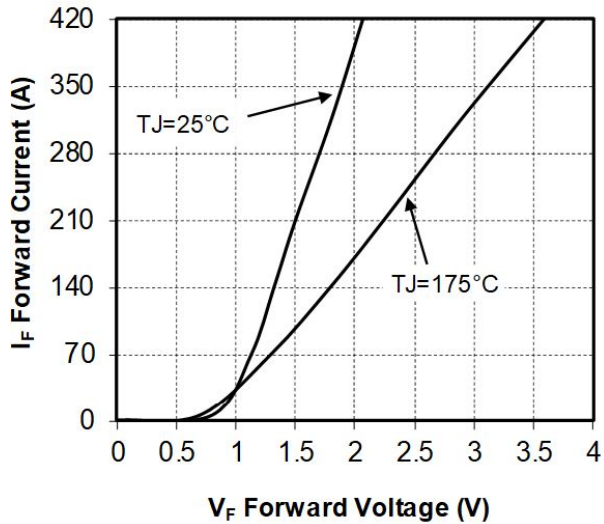
Figure 1-16. Forward Characteristics
