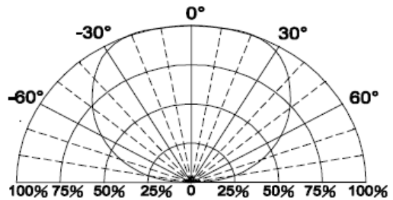
Fig.6 Directivity Radiation
